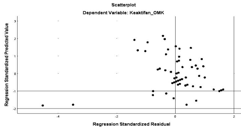
Gambar 5.2 Scatterplot
